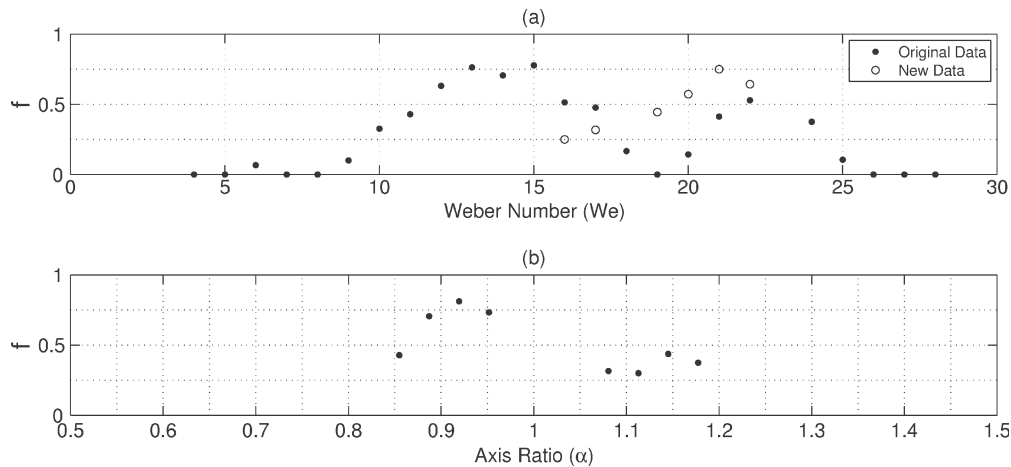
Figure 12. (a) Frequency of occurrence f of Mesler entrainment versus Weber number for drop impacts with new pipet tip superimposed over previous data. (b) Frequency of occurrence of Mesler entrainment versus \alpha for new drop impacts.
