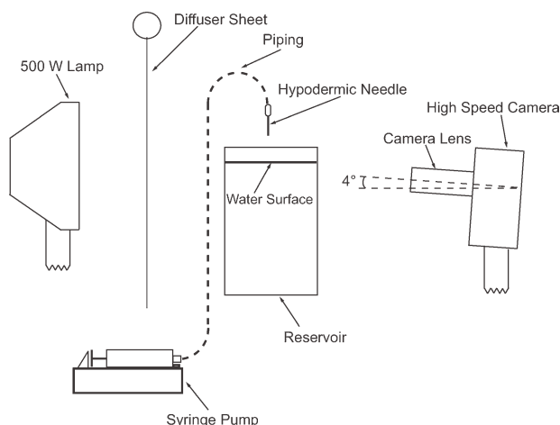
Figure 4. Apparatus used for recording drop impacts.
