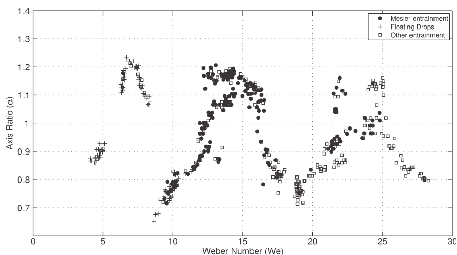
Figure 11. Plot of \alpha versus We for all drops.
