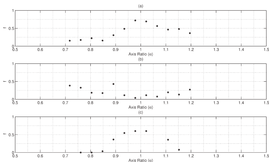
Figure 10. Plots of frequency of occurrence f of impact events versus axis ratio, \alpha for (a) Mesler entrainment, and (b) floating drops, (c) plot of f for Mesler entrainment versus \alpha using only data where We > 19 .
