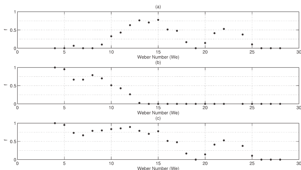
Figure 8. Plots of frequency of occurrence f of impact events versus Weber number We for (a) Mesler entrainment, (b) floating drops, and (c) Mesler entrainment or floating drops.
