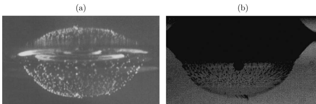
Figure 1. (a) Image taken from beneath the water surface of bubbles formed 10 ms after drop impact due to Sigler and Mesler; 5 (b) bubble formation pattern observed from beneath the water surface, due to the authors.
