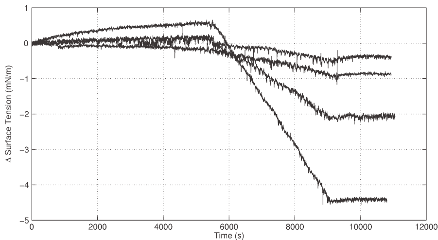
Figure 5. Change in surface tension of reservoir subjected to drop impacts at 6 drops/min for 1 hour for a Triton X-100 concentration of 0.1 mg/L.
