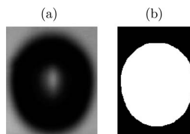
Figure 6. (a) Unprocessed drop image (cropped). (b) Processed drop image.
