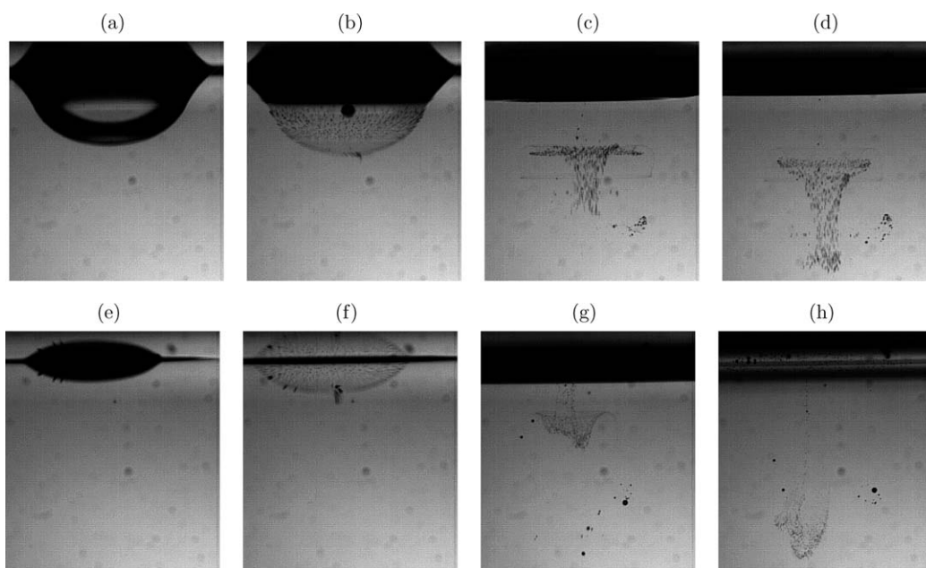
Figure 9. Images showing Mesler entrainment at (a–d) low Weber number We = 14 , and (e–h) high Weber number We = 21 .
