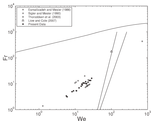
Figure 3. Plot showing the location of images obtained in the present study and in prior work in Froude versus Weber number space.
