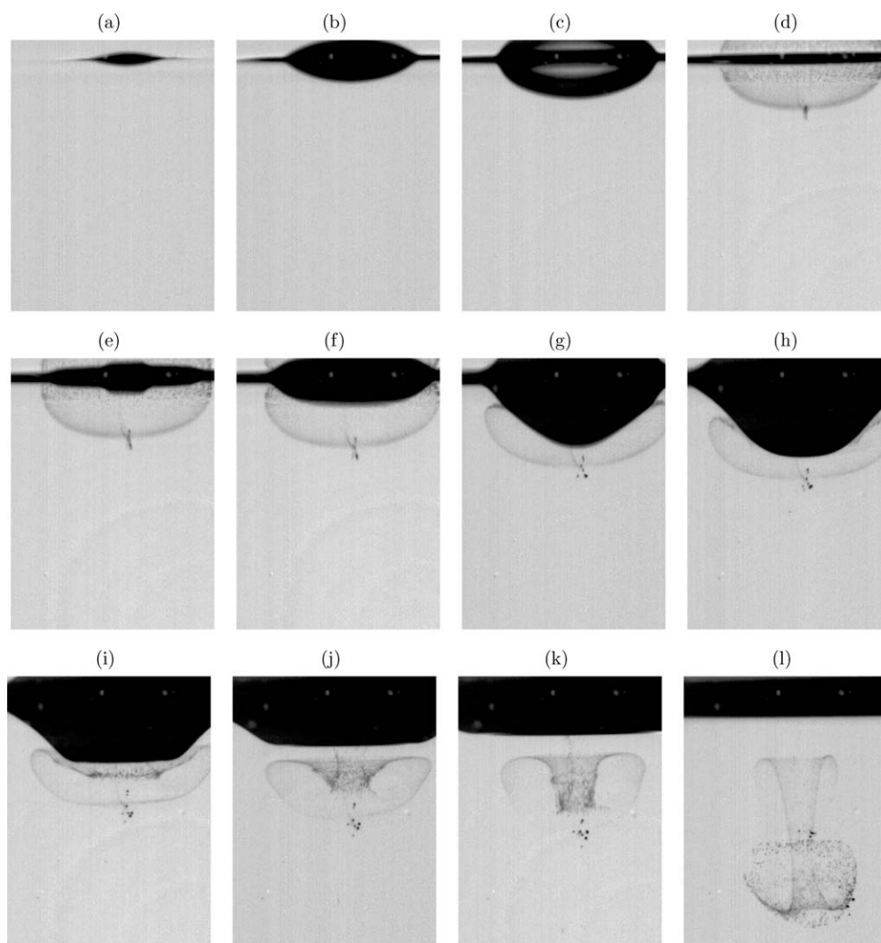
Figure 2. Sequence of images showing Mesler entrainment including the evolution of the crater, the formation of bubbles, and the subsequent convection of bubbles into the water bulk via the drop-formed vortex.
