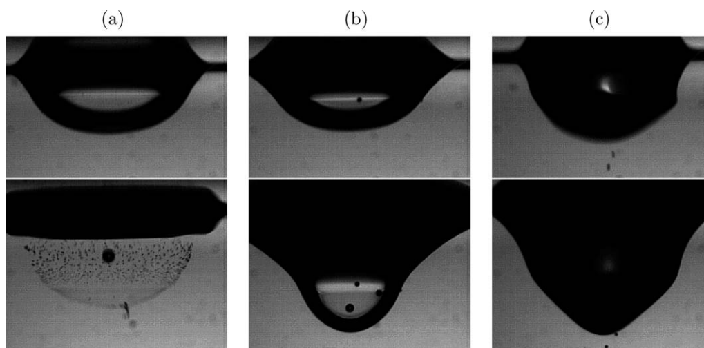
Figure 7. Three different impact scenarios observed: (a) Mesler entrainment, (b) floating or bouncing drop, and (c) other entrainment.
