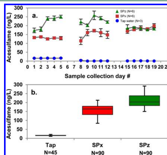
Figure 2. (a) Average ACE concentration detected in SPx, SPz ( N = 6 ), and tap water ( N = 3 ) samples per day over 3 weeks. (b) Box and whisker diagram for the average ACE concentration detected in SPx, SPz ( N = 90 ), and tap water ( N = 45 ) samples over 3 weeks.
