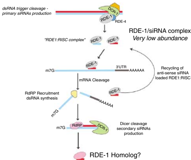
Figure 6 Function of rde-1 .
