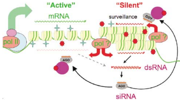
Figure 8 A chromatin–RNA feedback loop.
