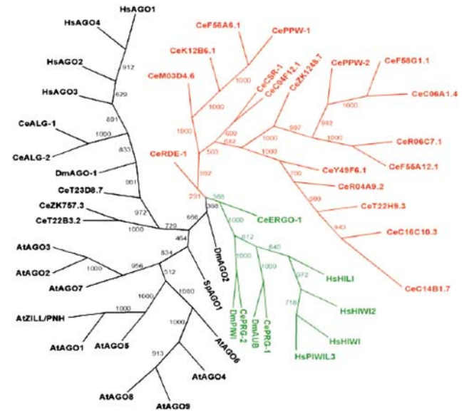
Figure 3 Phylogenetic tree of rde-1 -related genes (Argonaute family).
