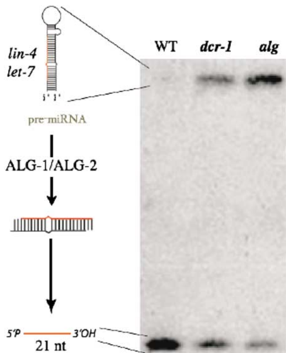
Figure 4 miRNA maturation. Gel electrophoretic separation.
